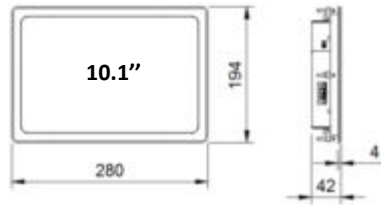
10.1" cut-out dimensions: 175mm x 261mm
