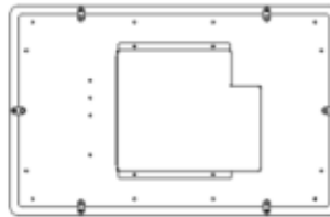
15.6" cut-out dimensions: 246mm x 398mm
