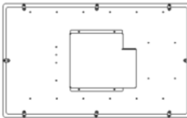
21.5" cut-out dimensions: 301mm x 511mm
