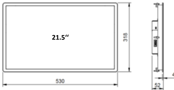
21.5" cut-out dimensions: 301mm x 511mm
