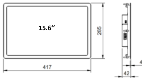
15.6" cut-out dimensions: 246mm x 398mm
