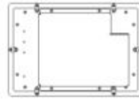
10.1" cut-out dimensions: 175mm x 261mm
