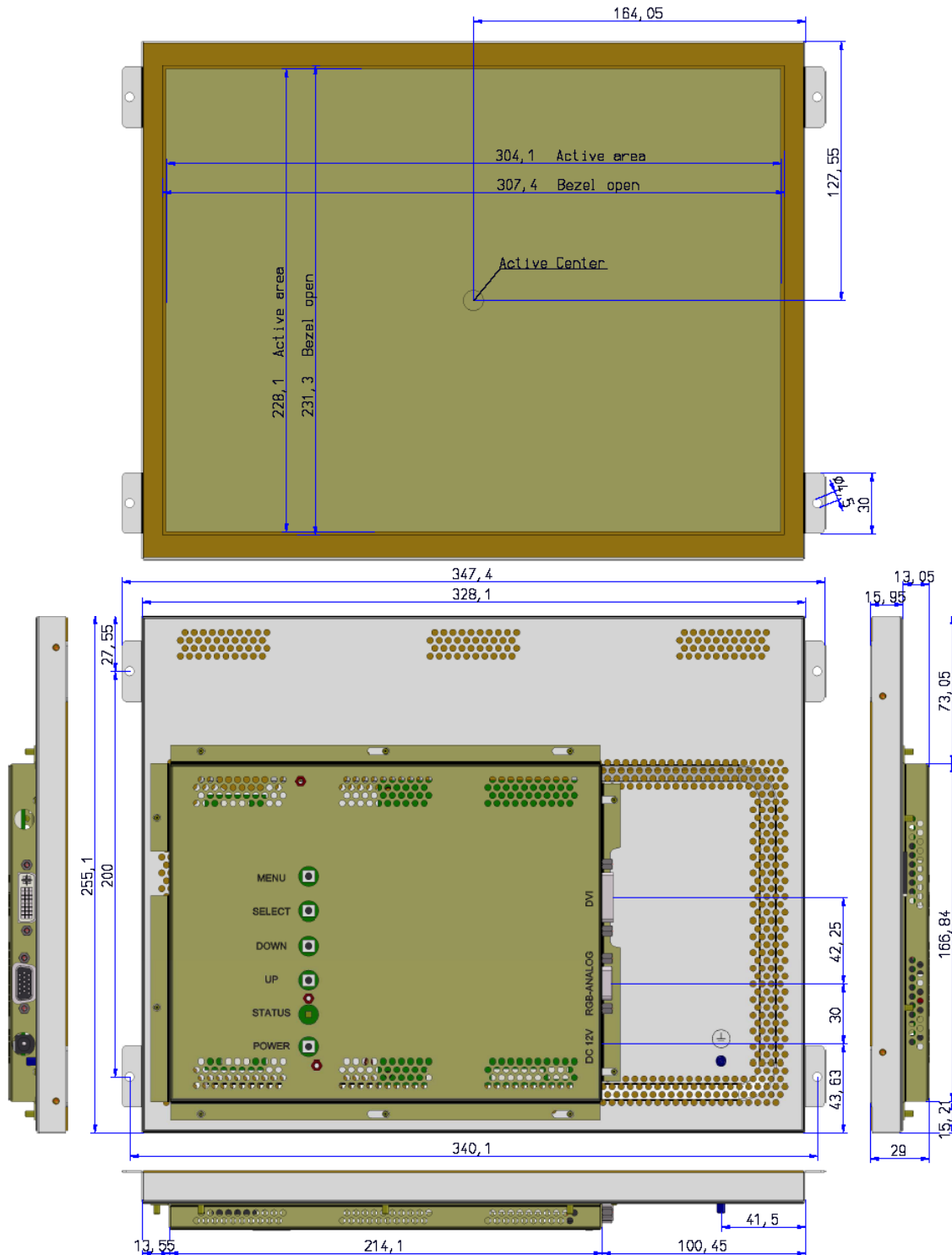
Figure 1: Mechanical Outlines
