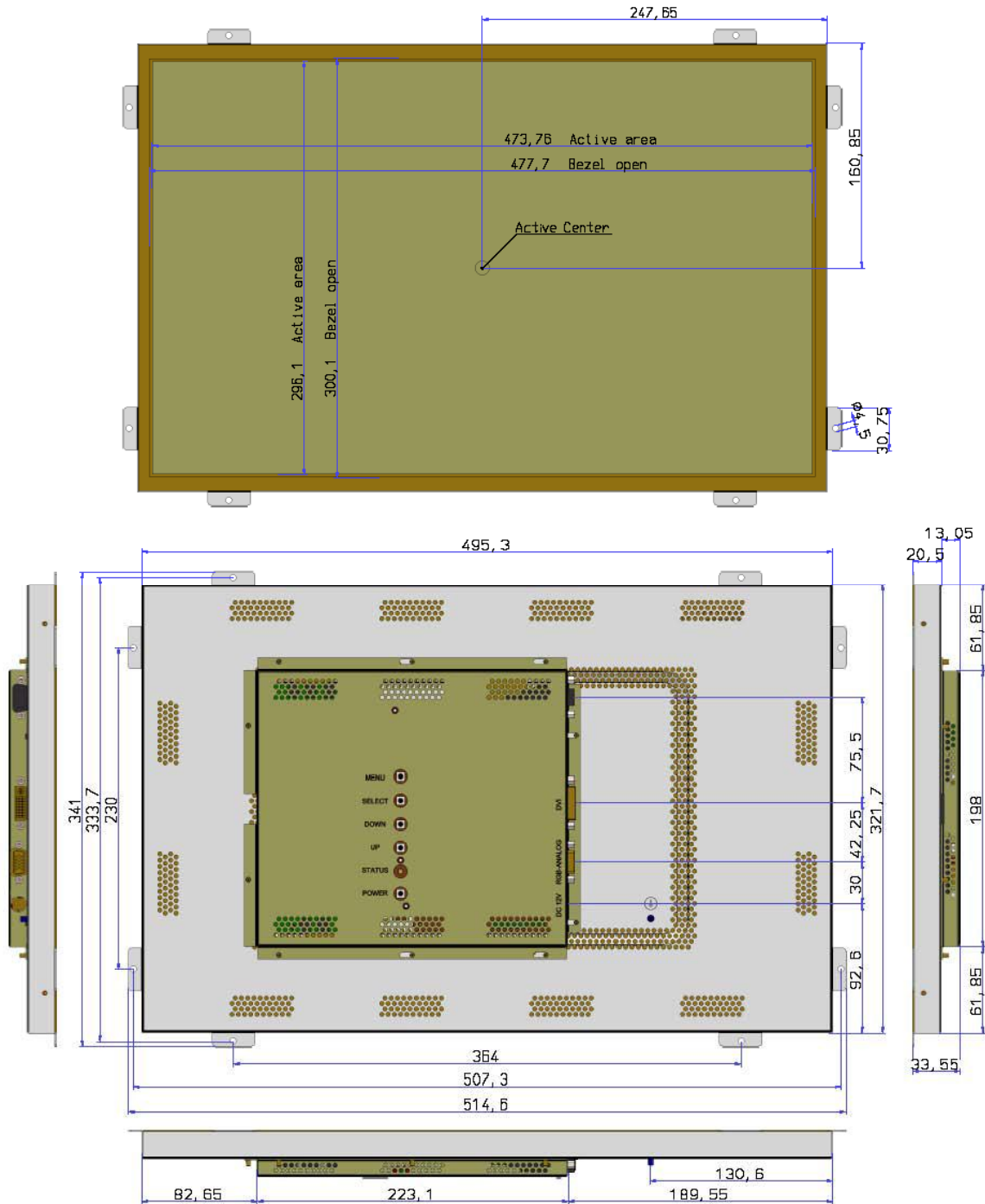
Figure 1: Mechanical Outlines
