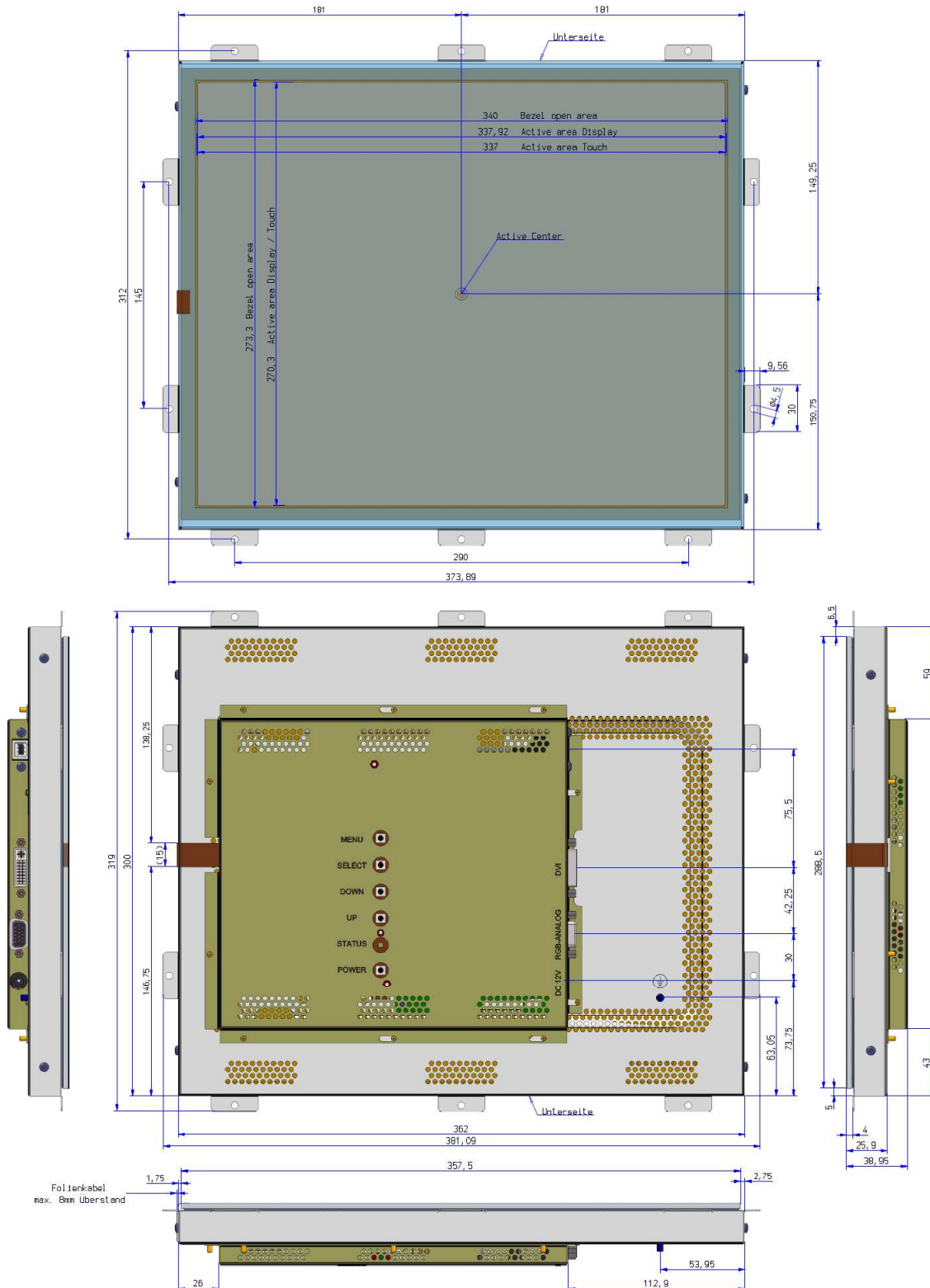
Figure 1: Mechanical Outlines
