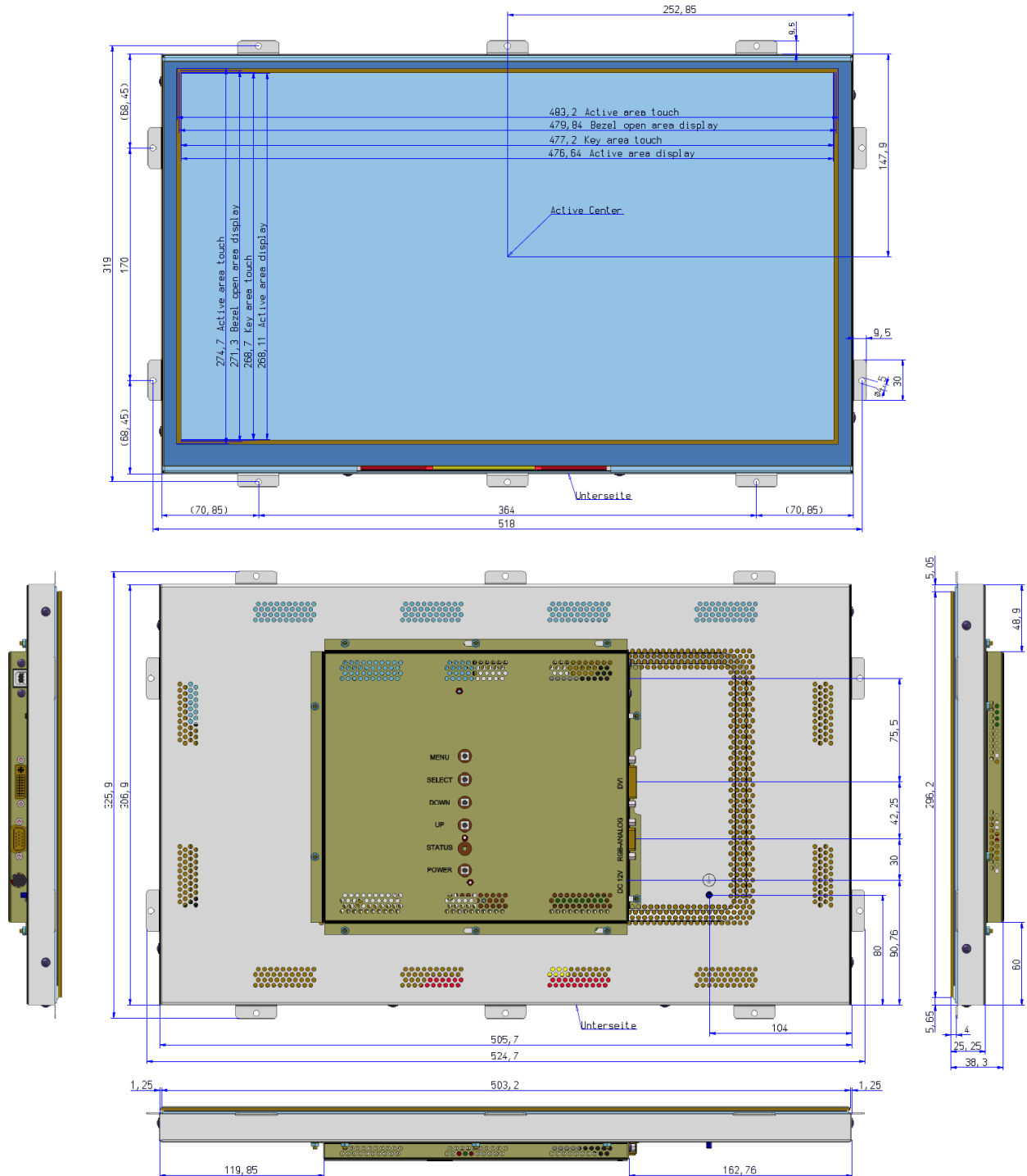
Figure 1: Mechanical Outlines
